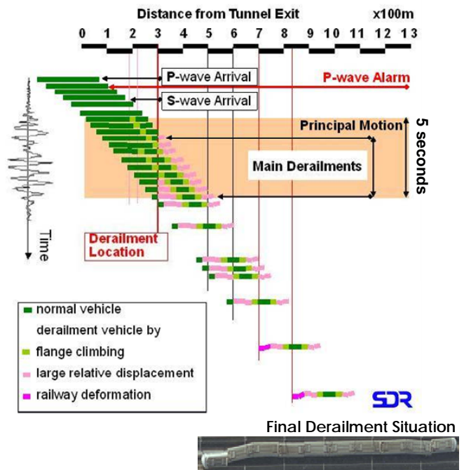
Fig.14 Performance of the deformation
