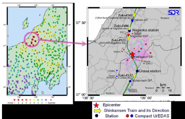
Fig.11 The 2004 Niigataken-Chuetsu Earthquake
