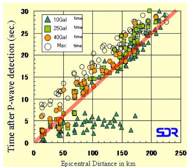
Fig.8 An example of alarm timings by simple triggers in case of the 2000 Tottoriken-Seibu Earthquake
