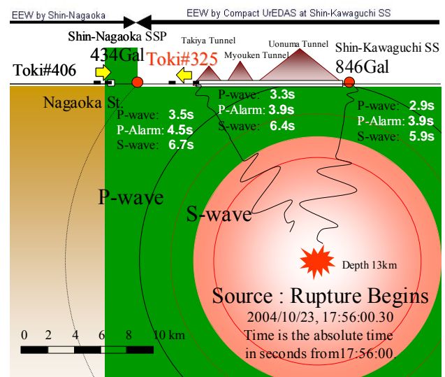
Fig.12 Schematic diagram for this earthquake
