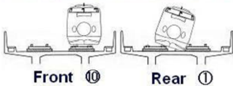
Fig.13 Detail of the derailment
