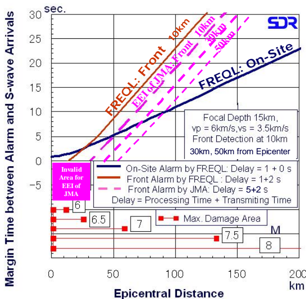
Fig.9 Margin time by EEW
