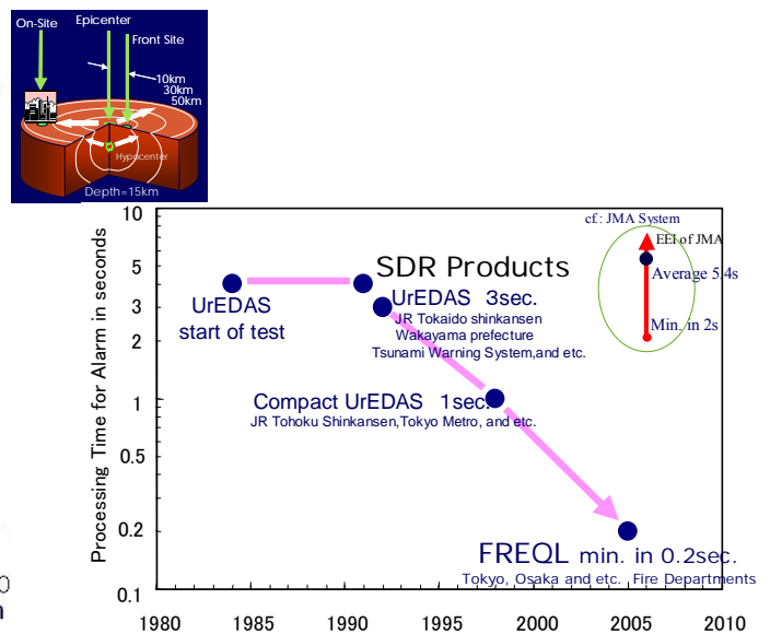
Fig.10 Change of processing time for EEW
