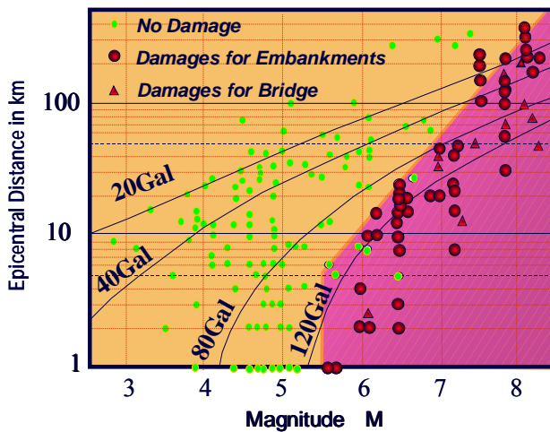
Fig.3 M- \Delta Diagram
