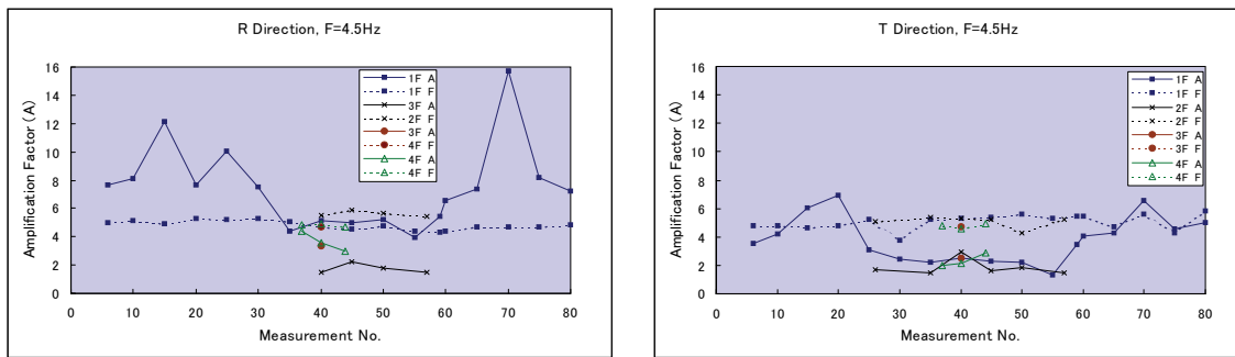
Figure 9: Distribution of amplification factor for R and T directions for F=4.5 Hz frequency.
