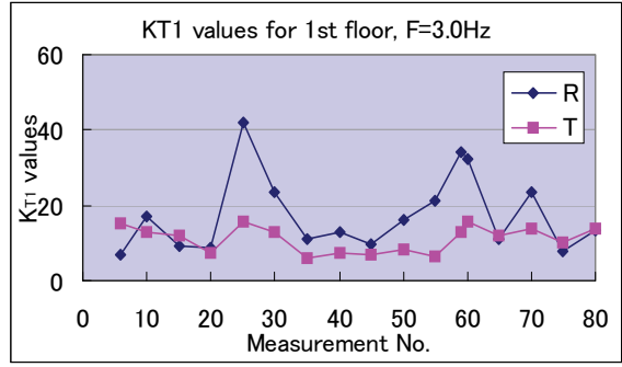
Figure 13: K_{T1} values for 1 st floor level, F=3.0 Hz
