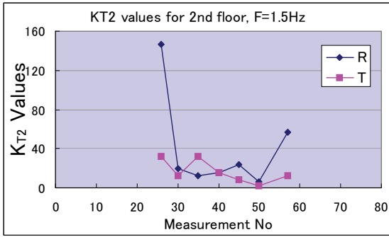
Figure 12: K_{T2} values for 2 nd floor level, F=1.5 Hz
