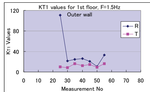
Figure 11: K_{T1} values for 1 st floor, F=1.5 Hz.
