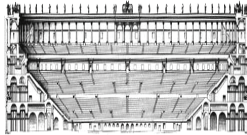
Figure 2: NS cross-section across the central axis of Colosseum.
